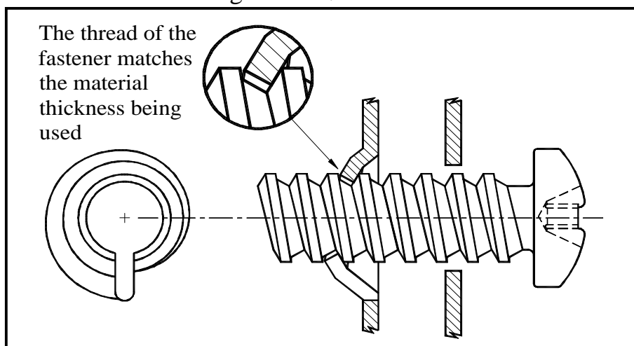
Pan-Flange
